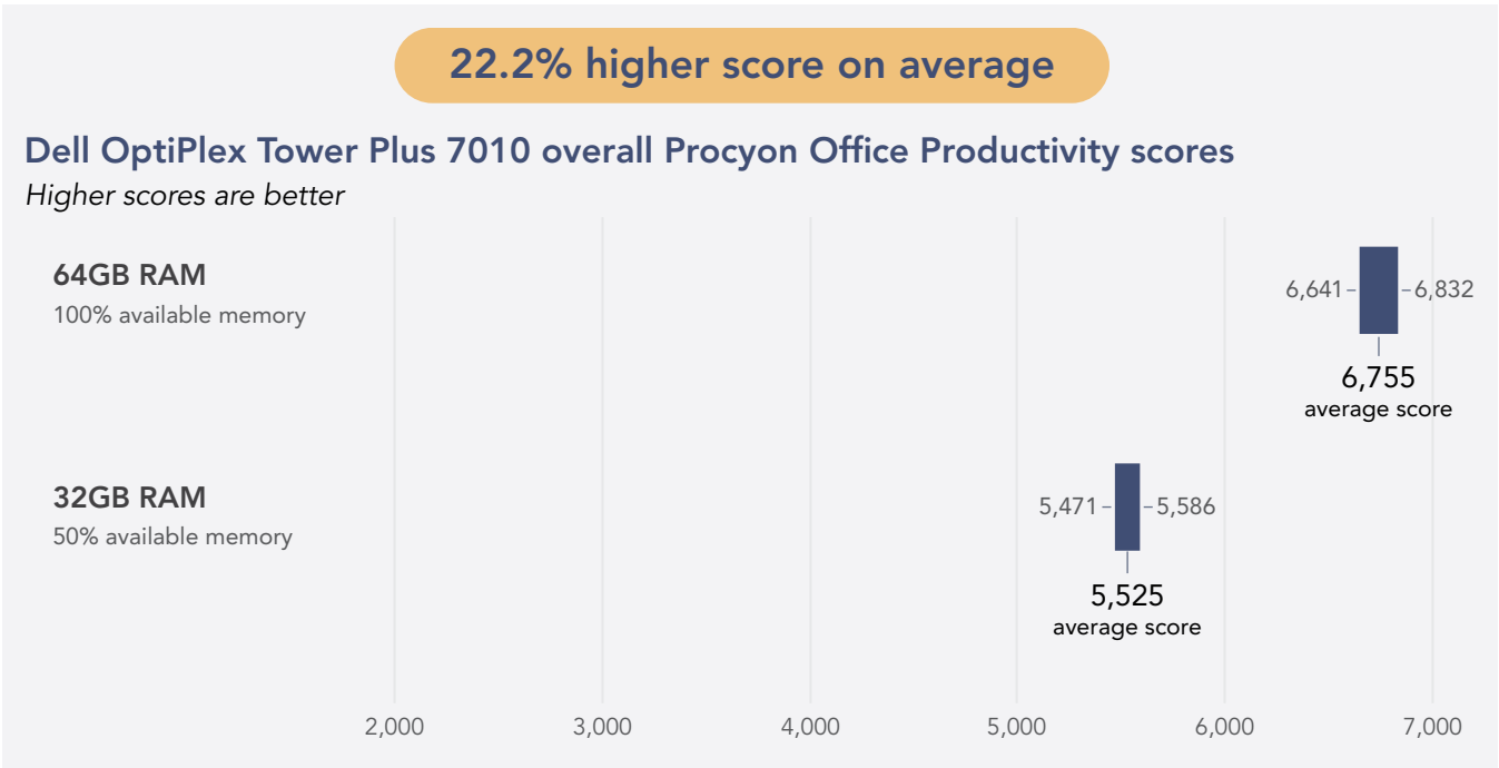
Figure 5: Procyon Office Productivity benchmark overall scores on the Dell OptiPlex Tower Plus 7010 with 64 GB of available memory and 32 GB of available memory. We show the range of three runs for each configuration. Higher scores are better. Source: Principled Technologies.
