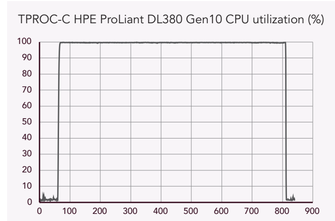
Figure 4: CPU utilization for the HPE ProLiant DL380 Gen10 server over the course of the TPROC-C test. Source: Principled Technologies.
