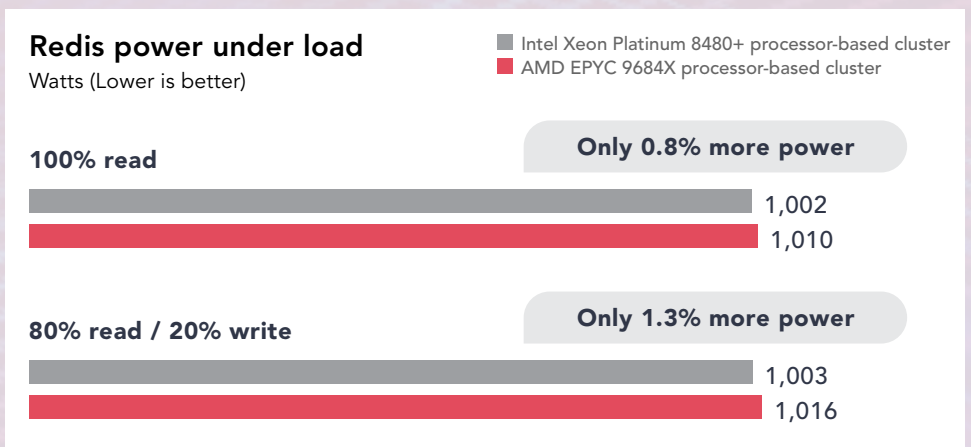
Figure 5: The power each solution consumed while running the workloads in the second scenario. Lower is better. Source: Principled Technologies.
