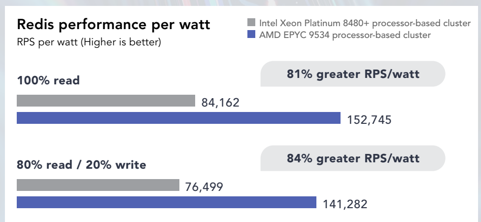
Figure 3: The performance per watt each solution delivered in the first test scenario under both I/O profiles. Higher is better. Source: Principled Technologies.
