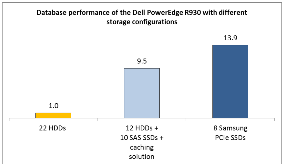
Figure 1: With Samsung NVMe storage configuration upgrades, the Dell PowerEdge R930 supported up to 13.9 times the performance of the all-HDD configuration.
