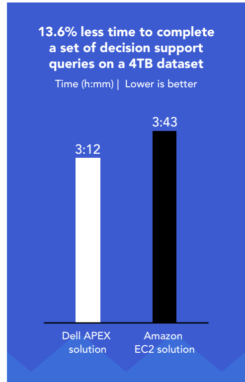
Figure 1: The total time that the Dell APEX solution and the Amazon EC2 c6i.16xlarge instances needed to complete the decision support workload we used in testing. Lower is better. Source: Principled Technologies.
